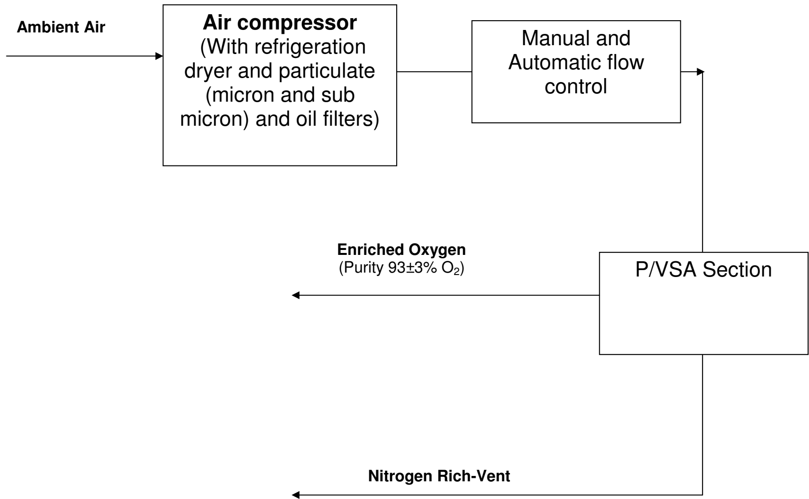
Figure-1: Block diagram proposed medical oxygen plant
