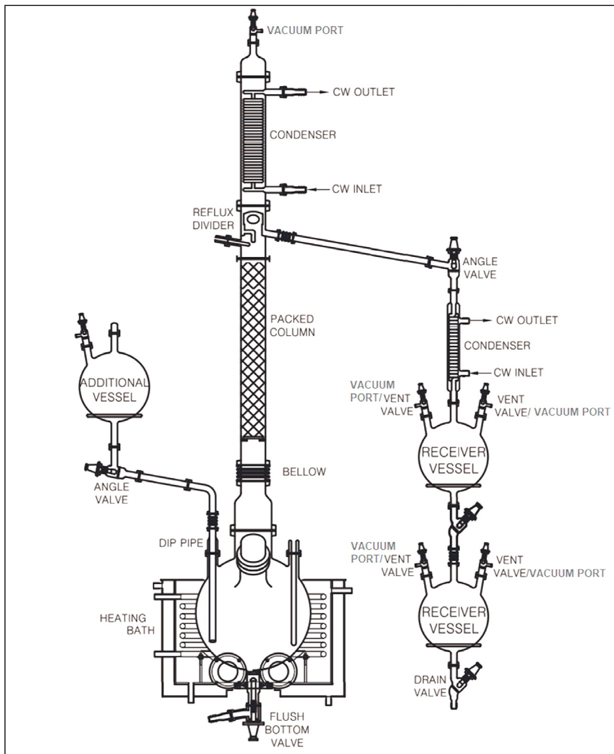
Semi-Automated High-Vacuum Fractional Distillation unit (Glass make)
