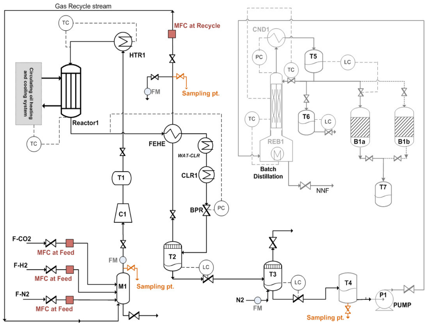
Figure1: Process Flow Scheme for 10Kg/day pilot plant
