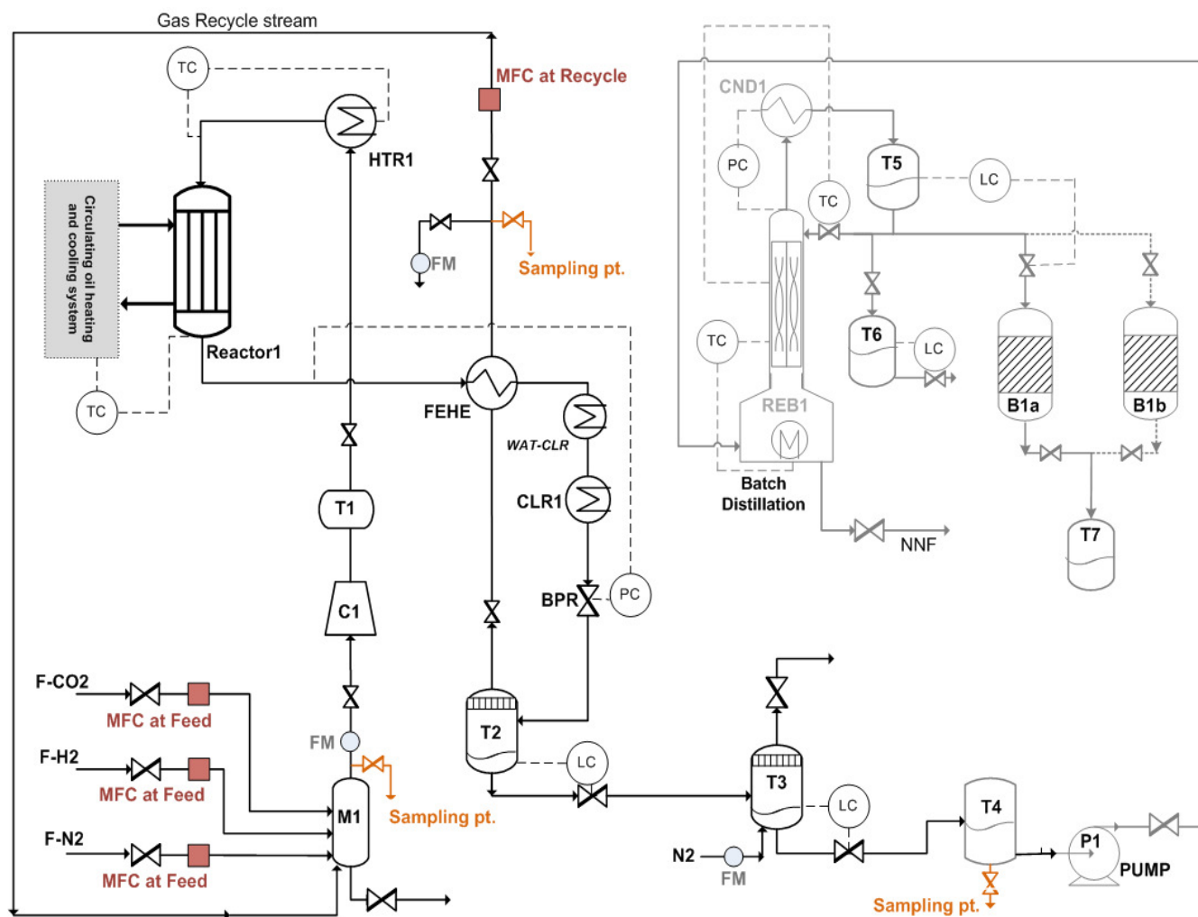
Figure1: Process Flow Scheme for 10Kg/day pilot plant
