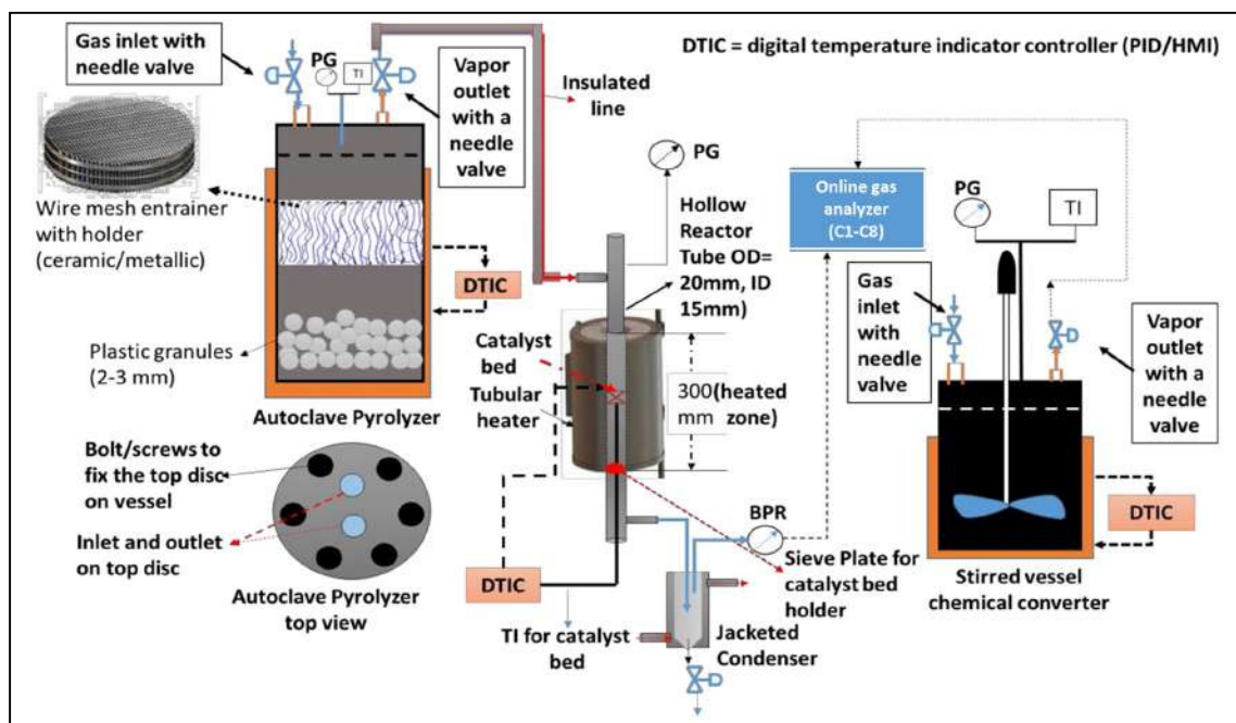
Fig.1: Schematics of Autoclave Pyrolyzer-Chemical Conversion system
